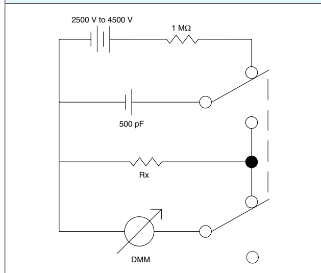
Figure 7 – ESD Test Description
