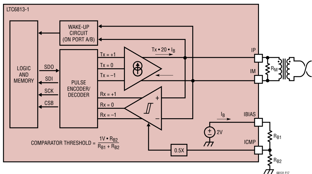
Figure 17. isoSPI Interface
