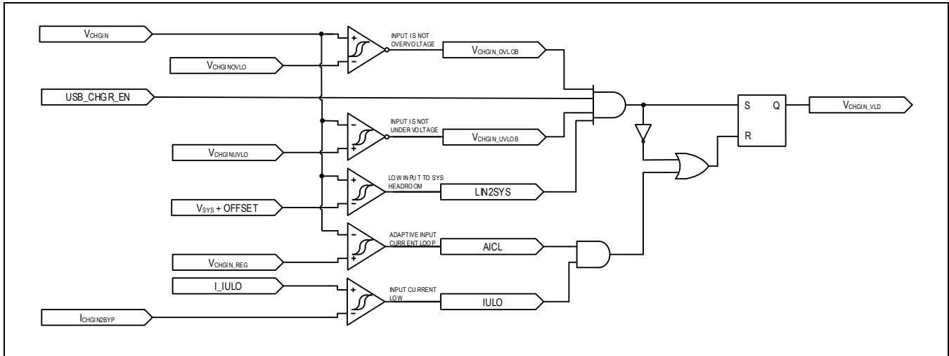
Figure 3. CHGIN Valid Signal Generation Logic
