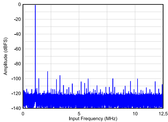
Figure 6-18. Single Tone FFT at F_{IN} = 1.1 MHz
