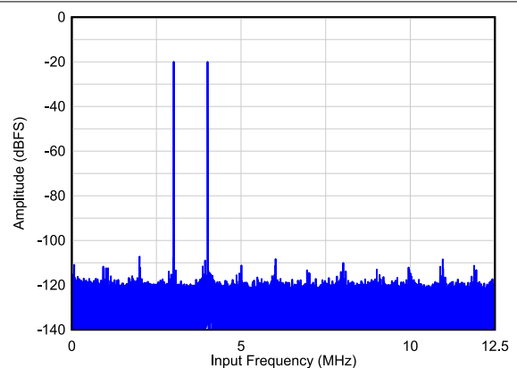
Figure 6-23. Two Tone FFT at F_{IN} = 3, 4 MHz
