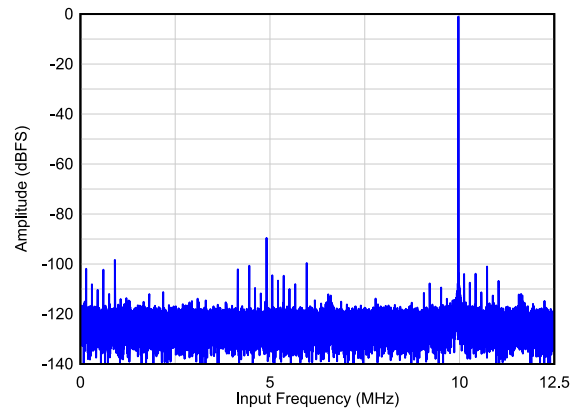
Figure 6-19. Single Tone FFT at F_{IN} = 10 MHz
