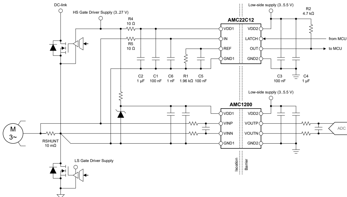
Figure 8-1. Using the AMC22C12 for Overcurrent Detection
