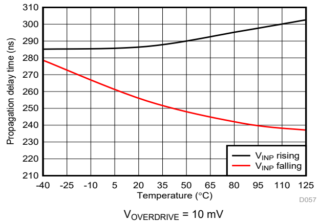
Figure 6-36. Cmp0 Propagation Delay vs Temperature
