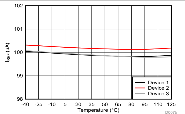
Figure 6-42. Reference Current vs Temperature
