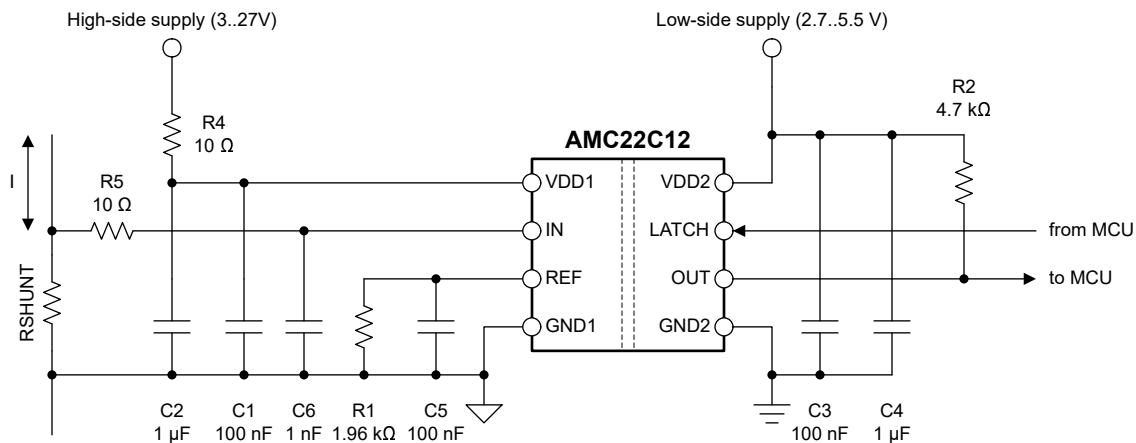
Figure 8-6. Decoupling of the AMC22C12
