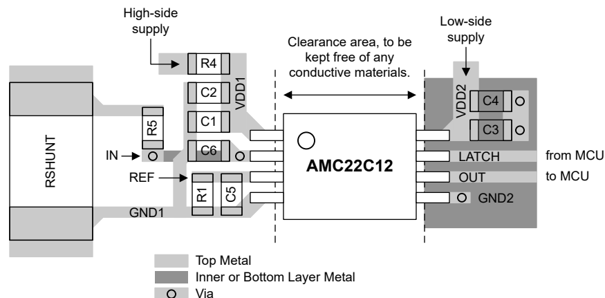
Figure 8-7. Recommended Layout of the AMC22C12
