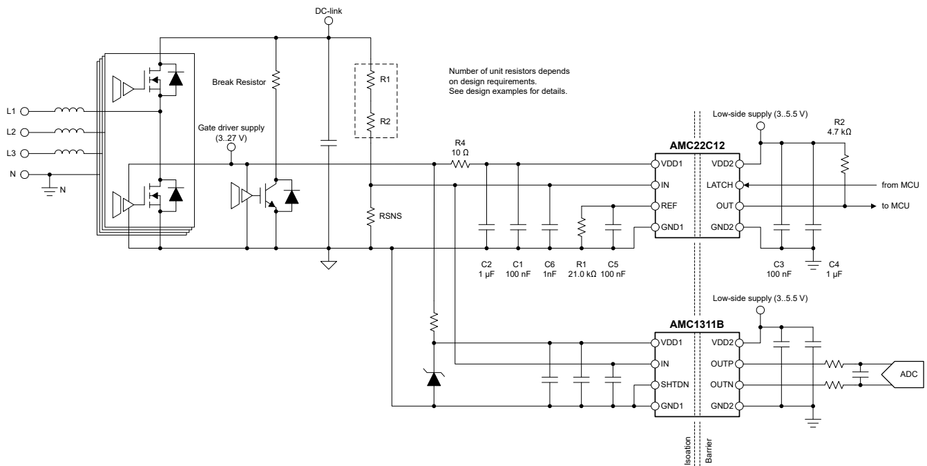
Figure 8-2. Using the AMC22C12 for Overvoltage Detection
