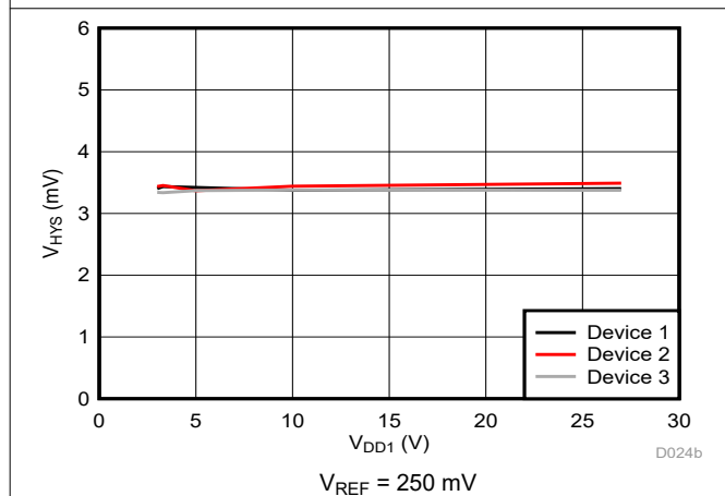
Figure 6-15. Cmp0 Trip Threshold Hysteresis vs Supply Voltage
