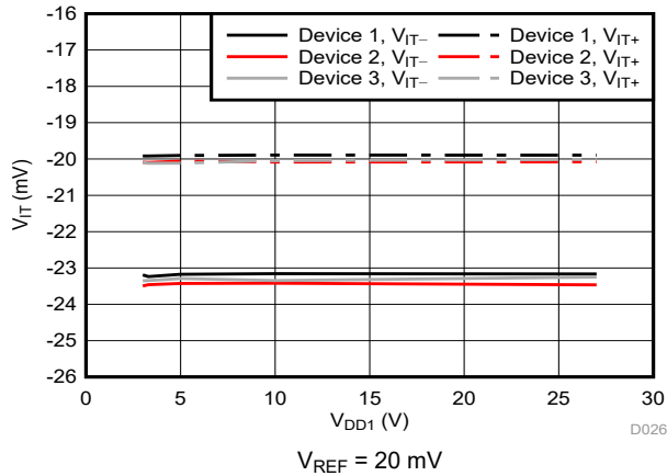
Figure 6-23. Cmp1 Trip Threshold vs Supply Voltage
