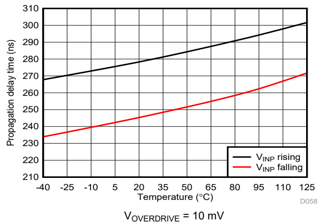
Figure 6-38. Cmp1 Propagation Delay vs Temperature
