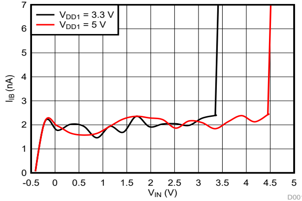
Figure 6-25. Input Bias Current vs Input Voltage
