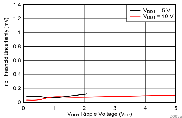
Figure 8-3. Trip Threshold Sensitivity to VDD1 Ripple Voltage (f RIPPLE = 10 kHz)
