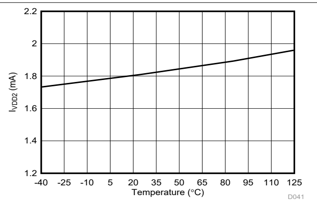
Figure 6-44. High-Side Supply Current vs Temperature
