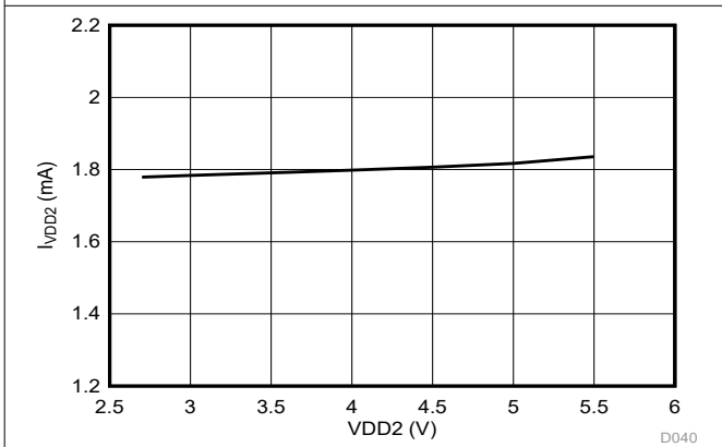
Figure 6-43. High-Side Supply Current vs Supply Voltage
