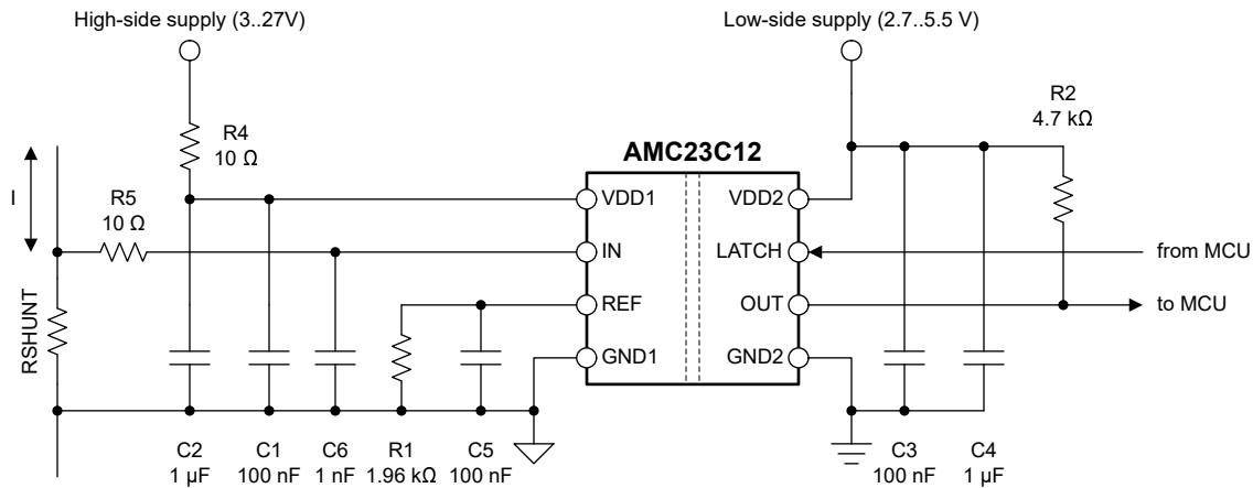
Figure 8-6. Decoupling of the AMC23C12
