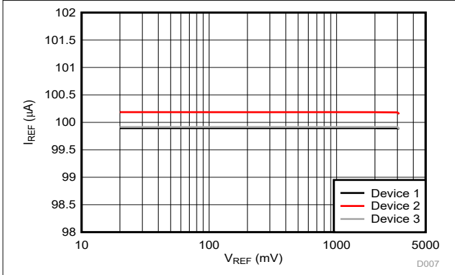
Figure 6-41. Reference Current vs Reference Voltage
