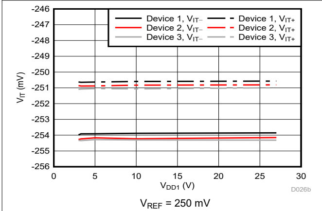
Figure 6-29. Cmp1 Trip Threshold vs Supply Voltage
