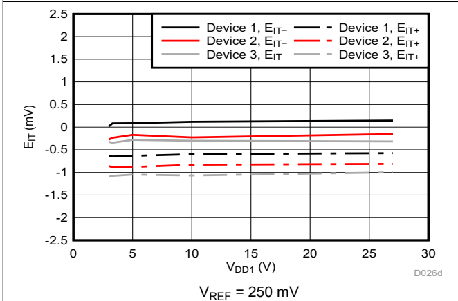
Figure 6-31. Cmp1 Trip Threshold Error vs Supply Voltage
