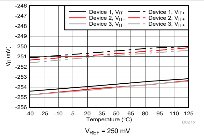
Figure 6-30. Cmp1 Trip Threshold vs Temperature
