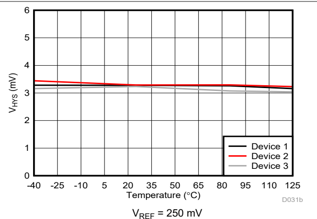
Figure 6-34. Cmp1 Trip Threshold Hysteresis vs Temperature
