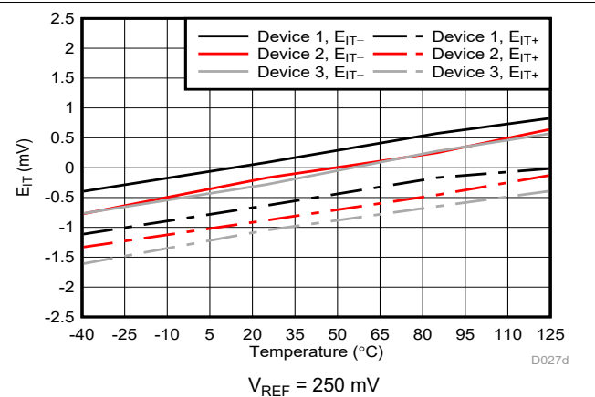
Figure 6-32. Cmp1 Trip Threshold Error vs Temperature
