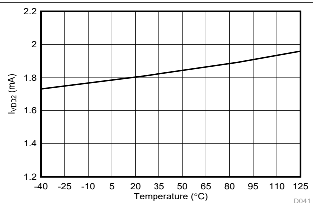
Figure 6-44. High-Side Supply Current vs Temperature
