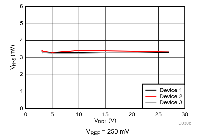
Figure 6-33. Cmp1 Trip Threshold Hysteresis vs Supply Voltage
