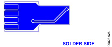
Figure 26. ADT7420FBZ Solder Side(Layer 2)
