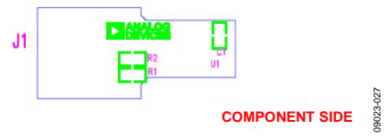
Figure 27. ADT7420FBZ Silkscreen
