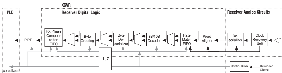
Figure 2–21. Receiver Channel PIPE \times 4 and \times 8 Modes
