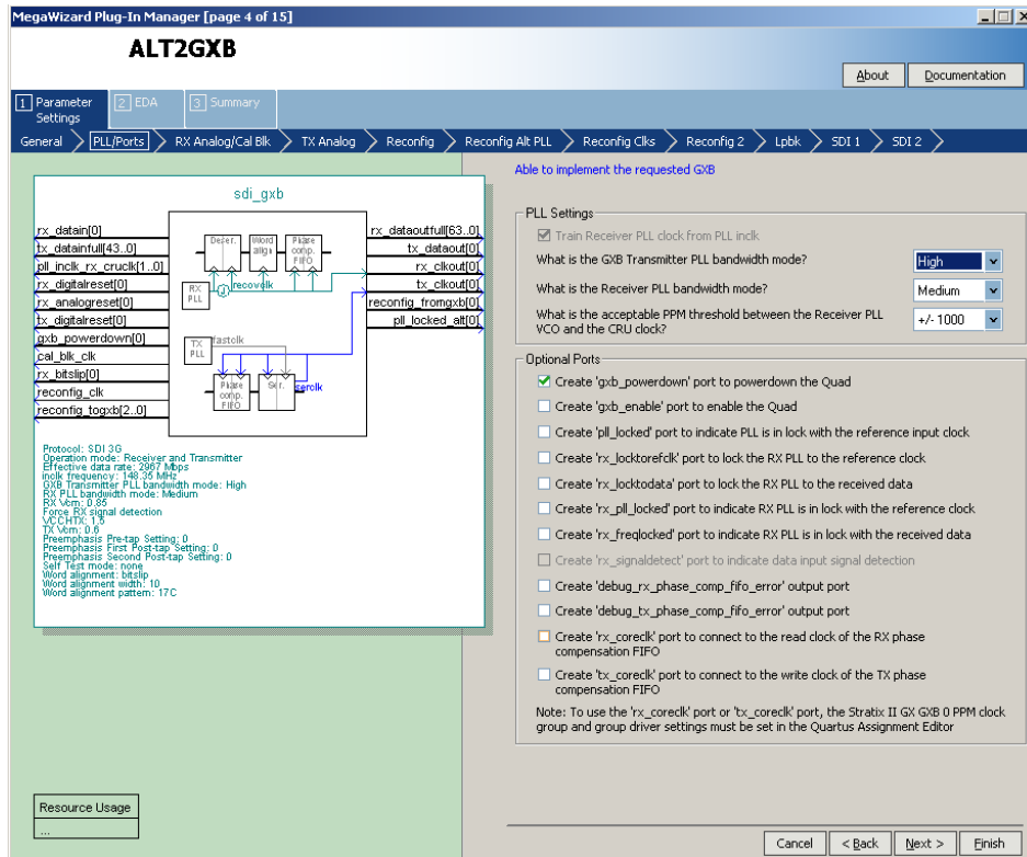
Figure 4-85. MegaWizard Plug-In Manager - ALT2GXB (PLL/Ports)
