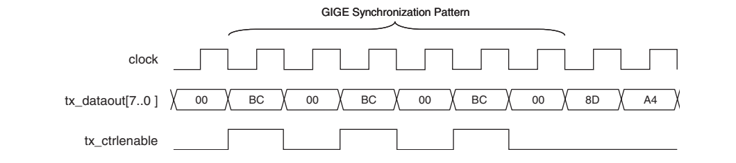
Figure 2–130. GIGE Synchronization Transmit Pattern
