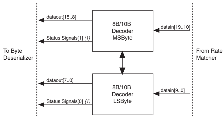
Figure 2–85. Active Data Path in Double-Width Mode
