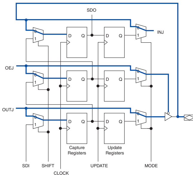
Figure 15–8. IEEE Std. 1149.1 BST SAMPLE/PRELOAD Mode
