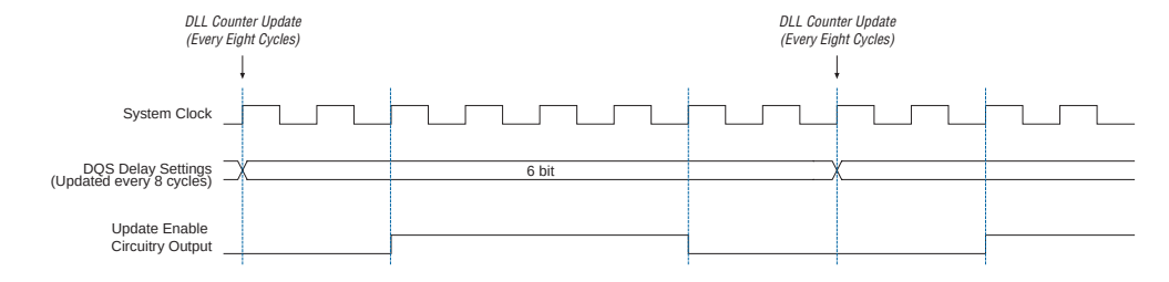
Figure 9–12. DQS Update Enable Waveform
