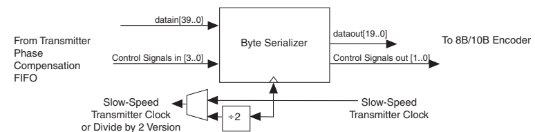
Figure 2–23. Byte Serializer
