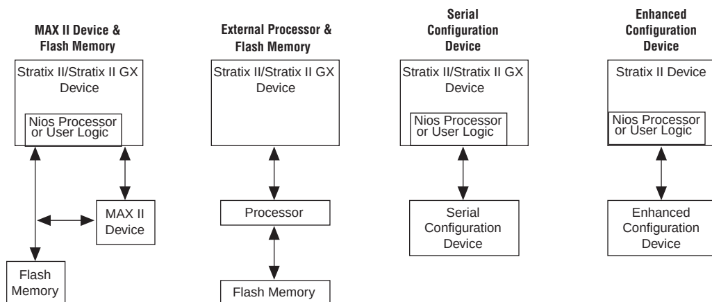
Figure 14–2. Remote System Upgrade Block Diagrams for Various Stratix II and Stratix II GX Configuration Schemes
