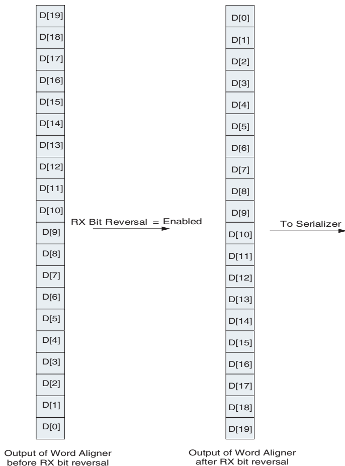
Figure 2–70. Receiver Bit Reversal in Double-Width Mode
