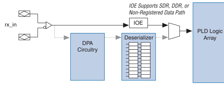
Figure 5-7. Deserializer Bypass
