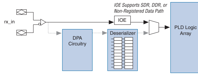
Figure 5-7. Deserializer Bypass
