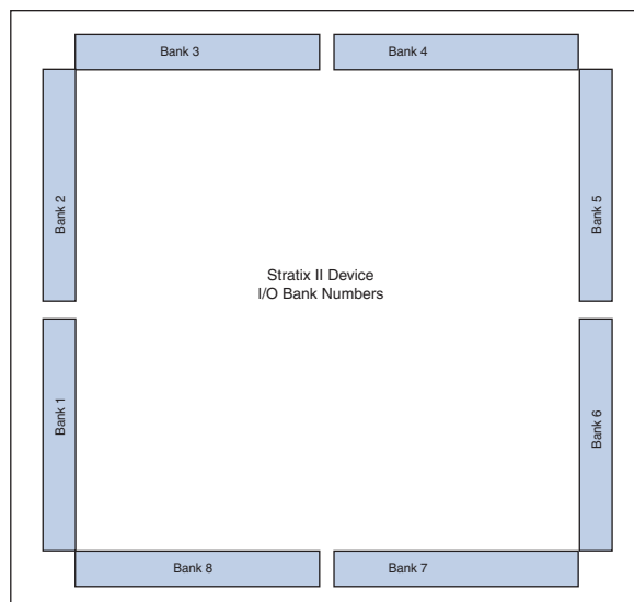
Figure 7–38. Stratix II I/O Bank Numbers
