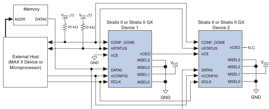
(1) The pull-up resistor should be connected to a supply that provides an acceptable input signal for all devices in the chain. V_{CC} should be high enough to meet the V_{IH} specification of the I/O on the device and the external host.
