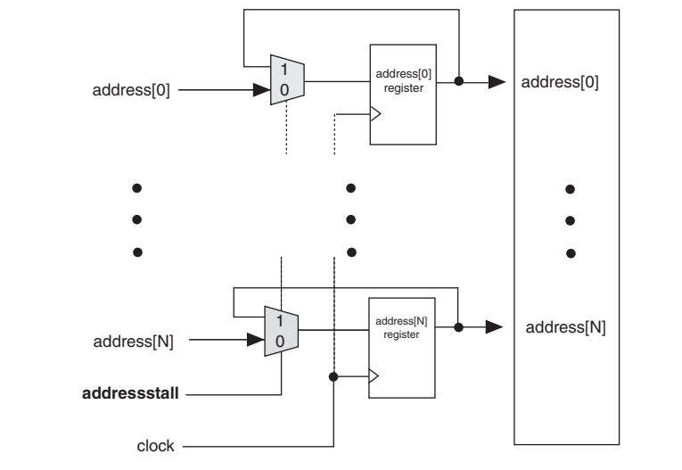
Figure 2-2. Stratix II and Stratix II GX Address Clock Enable Block Diagram
