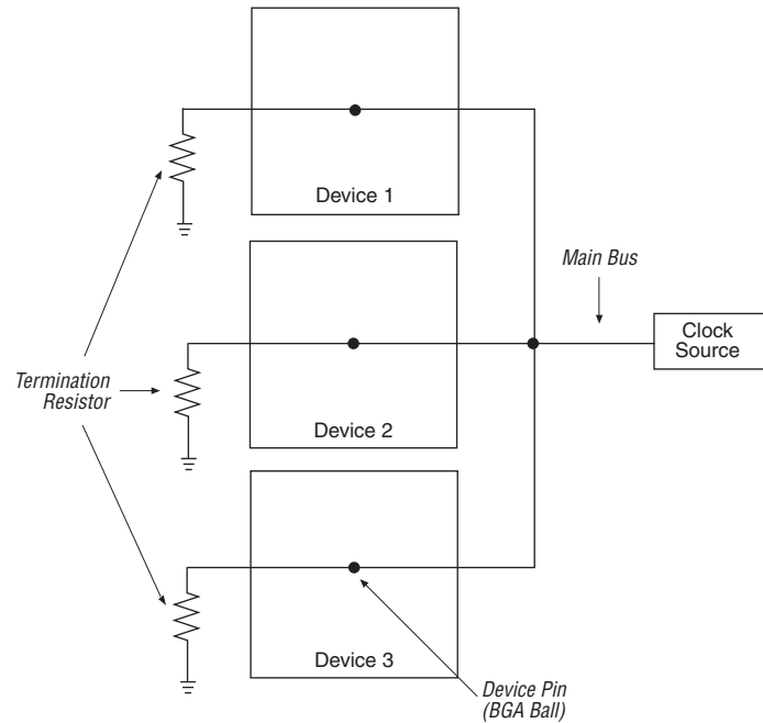
Figure 11–19. Star Routing
