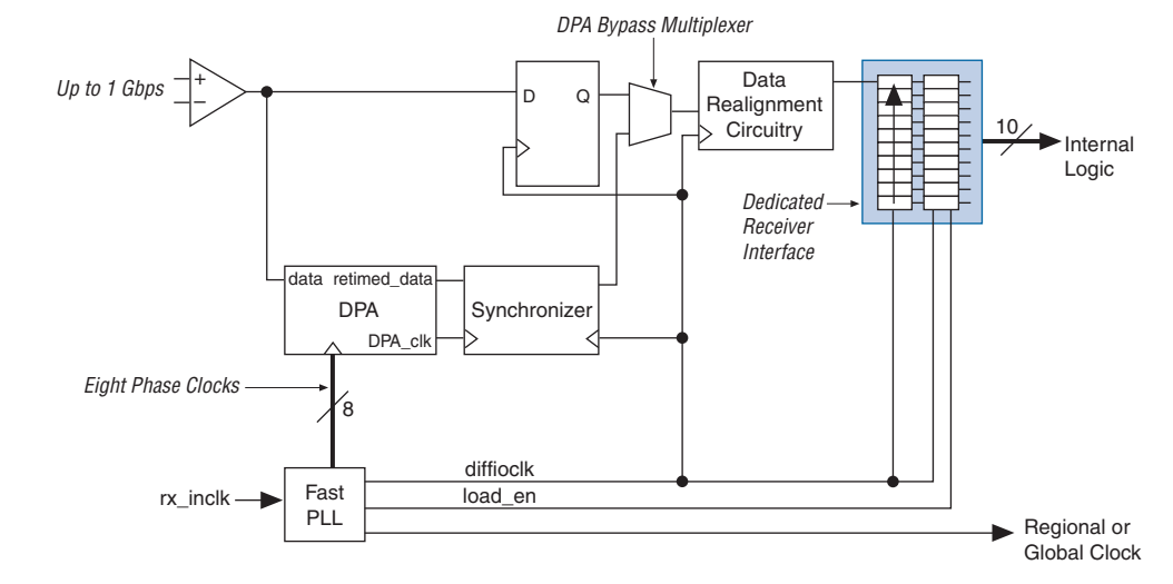
Figure 5–6. Receiver Block Diagram
