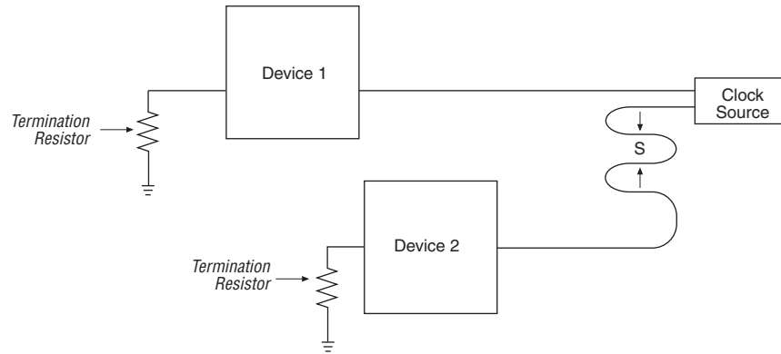
Figure 11–20. Serpentine Routing
