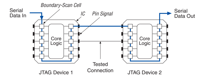
Figure 9-1. IEEE Std. 1149.1 Boundary-Scan Testing
