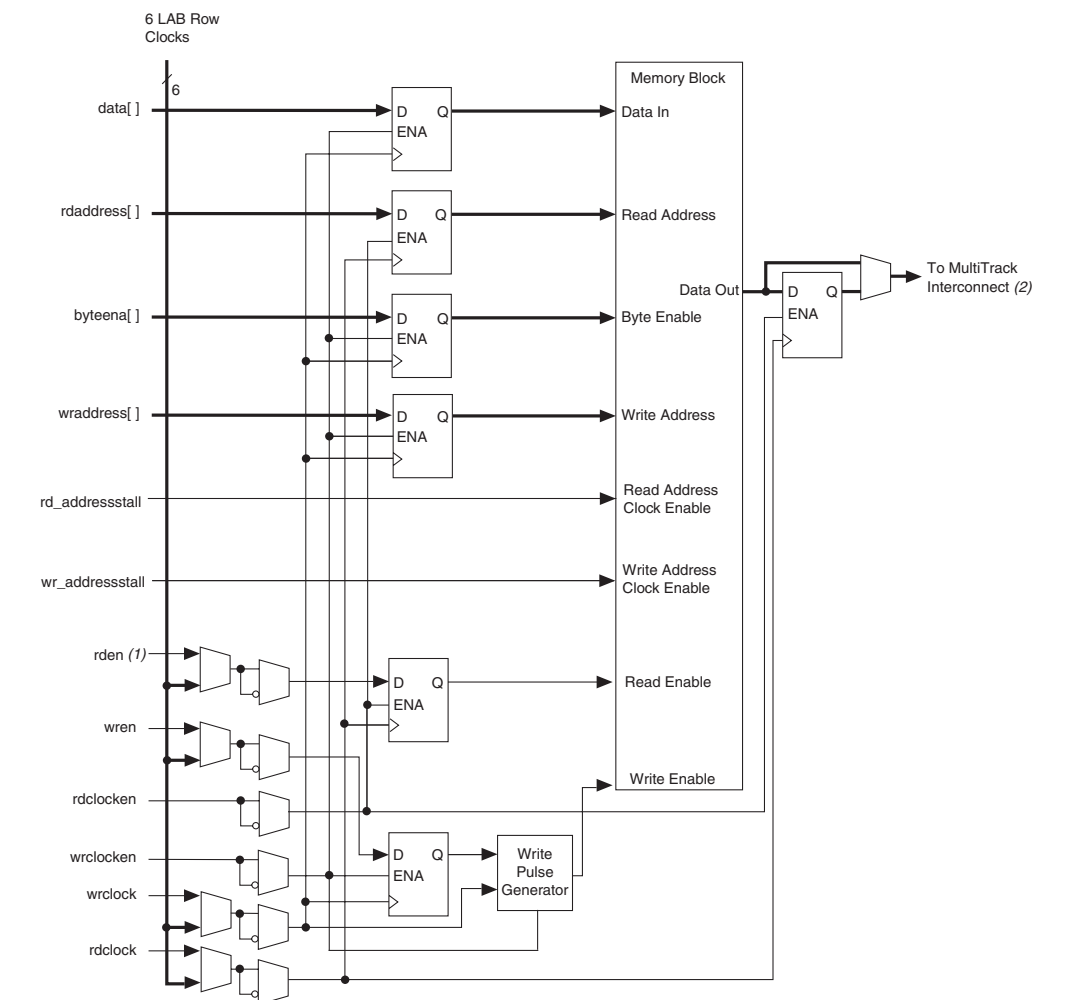
Figure 8–17. Cyclone II Read/Write Clock Mode Notes (1), (2)
