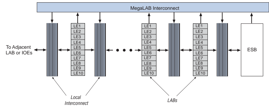
Figure 2. MegaLAB Structure
