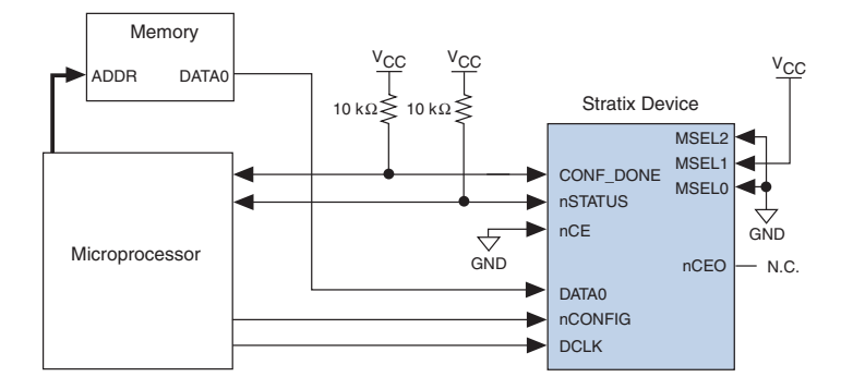
Figure 1–8. PS Configuration Circuit with Microprocessor
