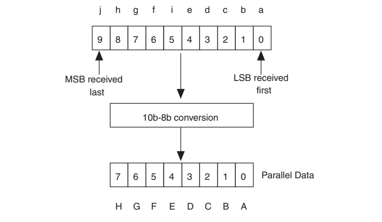
Figure 6–12. 10-Bit to 8-Bit Conversion
