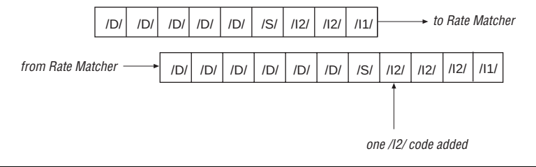
Figure 6–11. Addition of an /I2/ Ordered Set During an Almost Empty Condition
