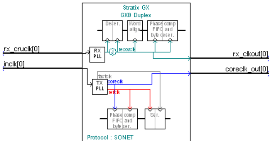
Figure 4–12. altqxb Megafunction in SOMET Mode With Train Receiver CRU From Transmitter PLL Disabled
