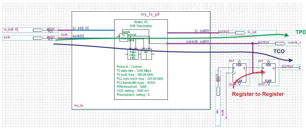
Figure 5–1. Transmit PLL coreclk_out Showing t_{PD} & t_{CD} Registers
