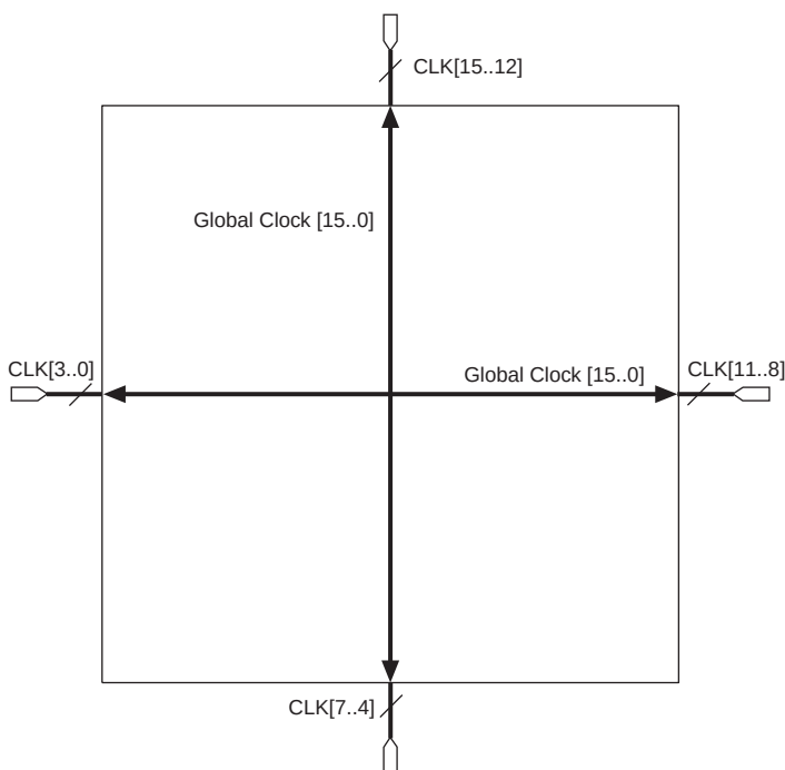
Figure 13–19. Global Clocking
