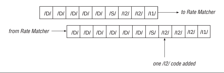
Figure 6–11. Addition of an /I2/ Ordered Set During an Almost Empty Condition
