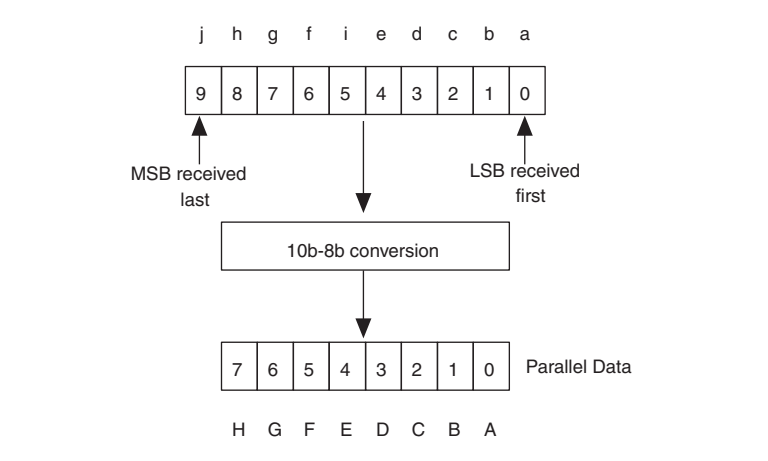
Figure 6–12. 10-Bit to 8-Bit Conversion
