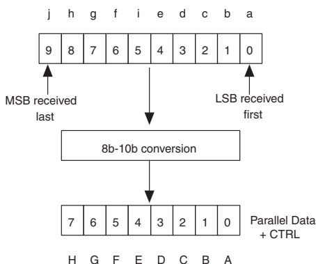
Figure 5–9. 10-Bit to 8-Bit Conversion
