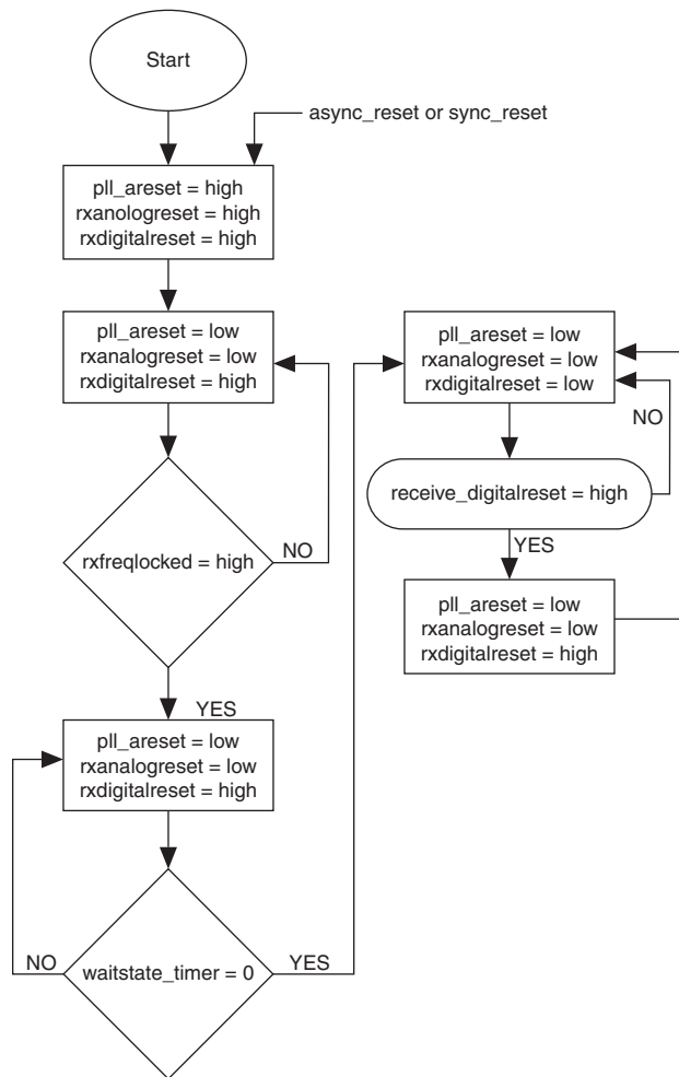
Figure 9–11. Receiver Reset Sequence
