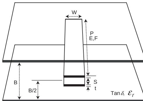
Figure 4–32. Broadside-Coupled Differential Stripline
