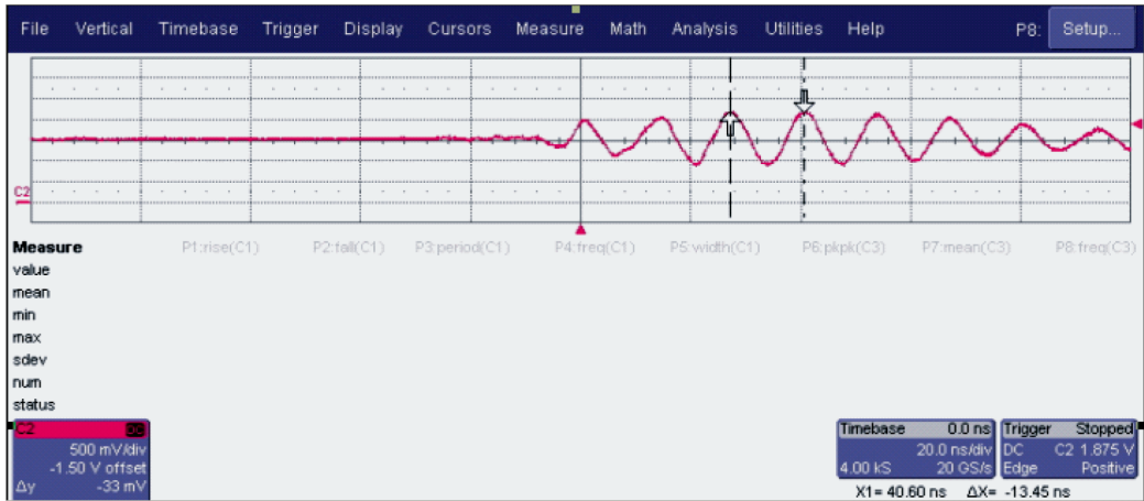
Figure 4–8. Excessive Ripple at the Output of a Switching Regulator
