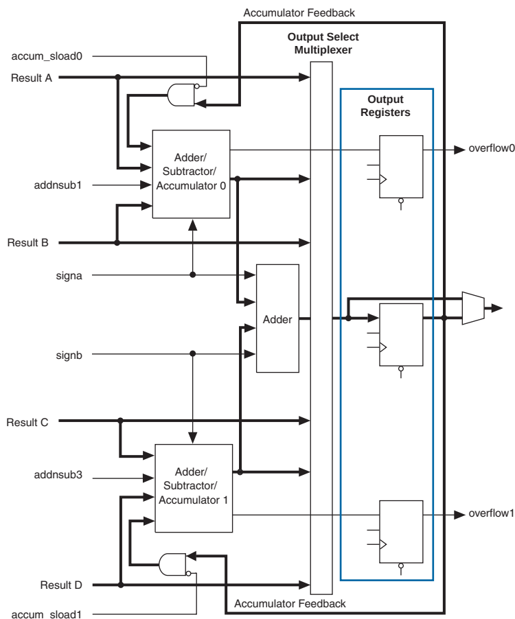
Figure 6–5. Adder/Output Block
