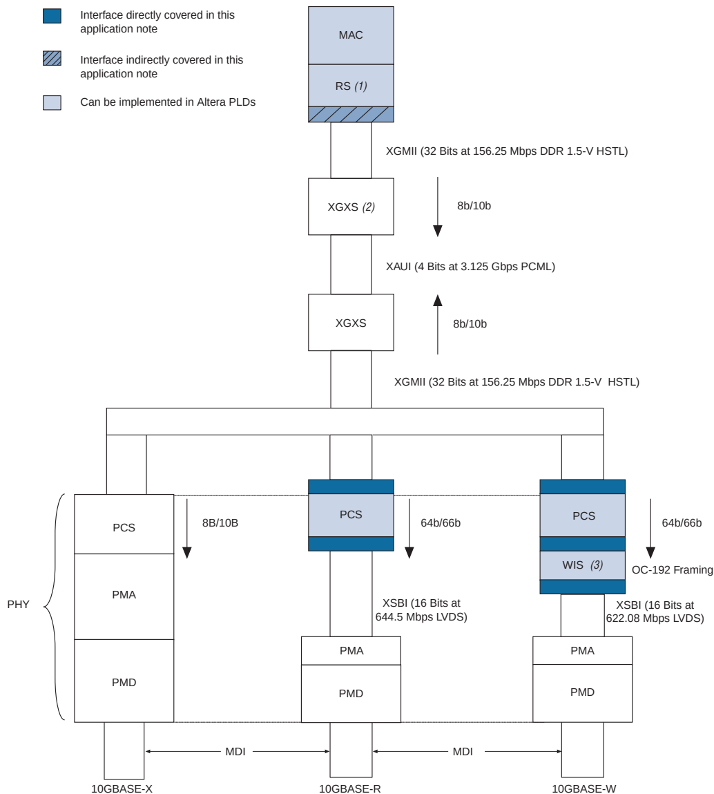
Figure 8–2. 10-Gigabit Ethernet Block Diagram
