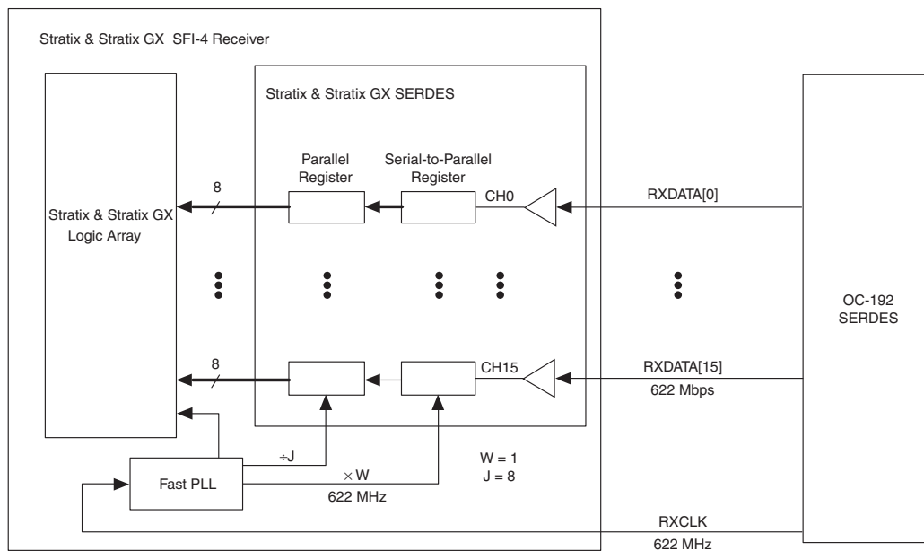
Figure 9–6. Framing Receiver Interface in Stratix & Stratix GX Devices
