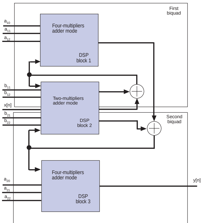
Figure 7-23. Two Cascaded Biquads
