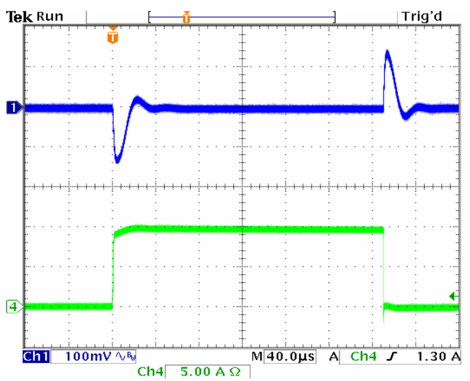
Transient Response: 5V IN /3.3V OUT , 0-9A, 7A/µS, C OUT = 5x22µF
