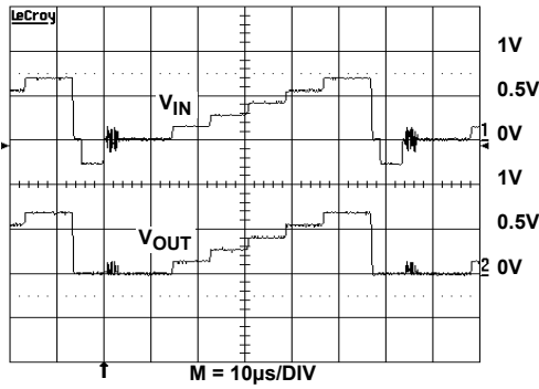
FIGURE 30. VIDEO SIGNAL
