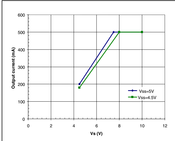
Figure 8. Maximum output current vs. reference voltage (DAC=100%)
