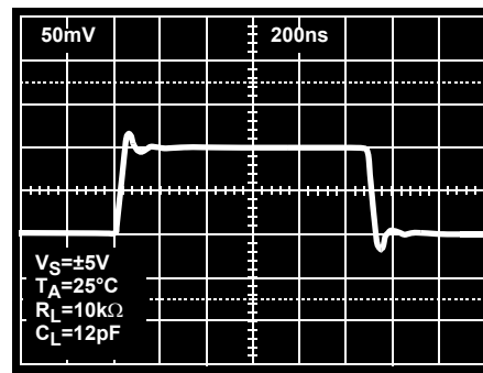
FIGURE 22. SMALL SIGNAL TRANSIENT REPOSNE
