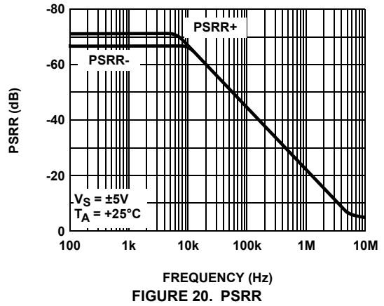
FIGURE 20. PSRR
