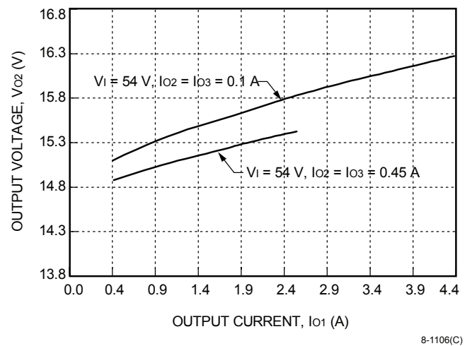
Figure 8. DW025ACL-M Typical Cross Regulation with Respect to I_{o1}
