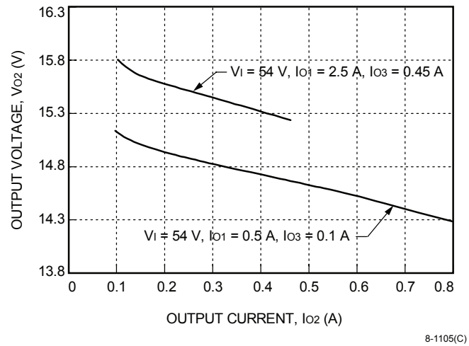
Figure 7. DW025ACL-M Typical Load Regulation
