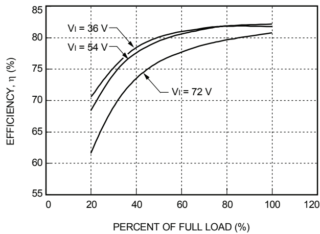
Figure 13. DW025ABK-M Typical Converter Efficiency
