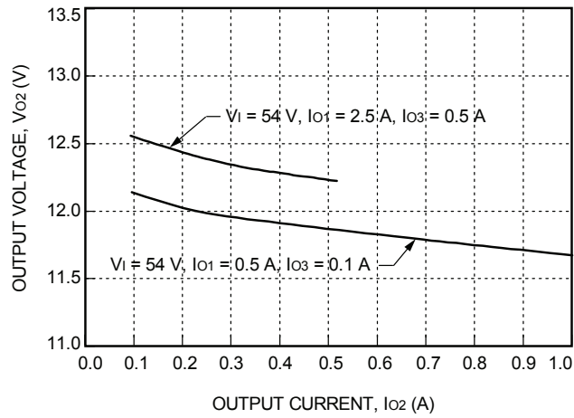
Figure 5. DW025ABK-M Typical Load Regulation
