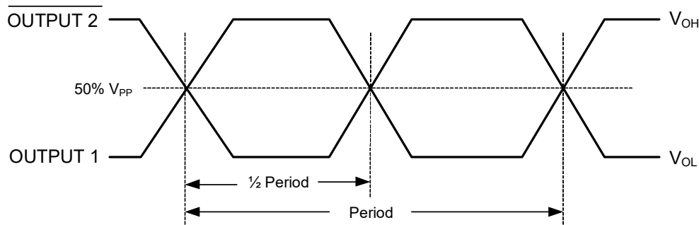
Oscillator Symmetry
