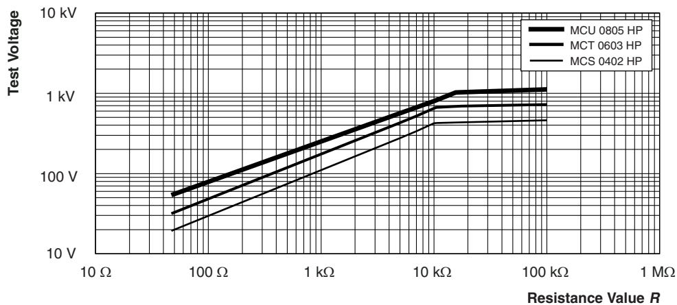
Pulse load rating in accordance with EN 60115-1 clause 4.27; 1.2 \mu s/50 \mu s; 5 pulses at 12 s interval; for permissible resistance change \pm (0.5 \% R + 0.05 \Omega)
