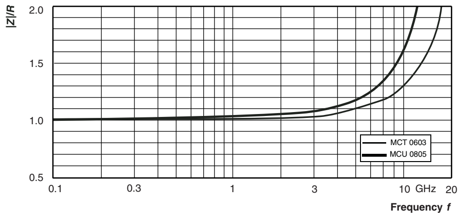
Relative impedance for 49.9 \Omega chip resistor
