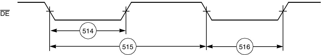
Figure 2-32. OnCE—Debug Request
