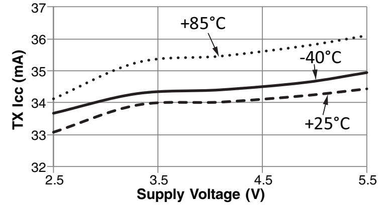
Figure 8: NT Series Transceiver TX Current Consumption vs. Supply Voltage at +12.5dBm
