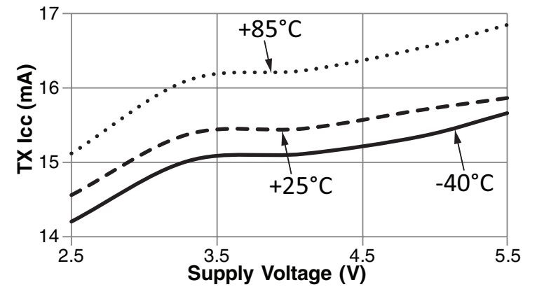
Figure 9: NT Series Transceiver TX Current Consumption vs. Supply Voltage at 0dBm
