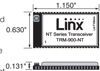
Figure 1: Package Dimensions
