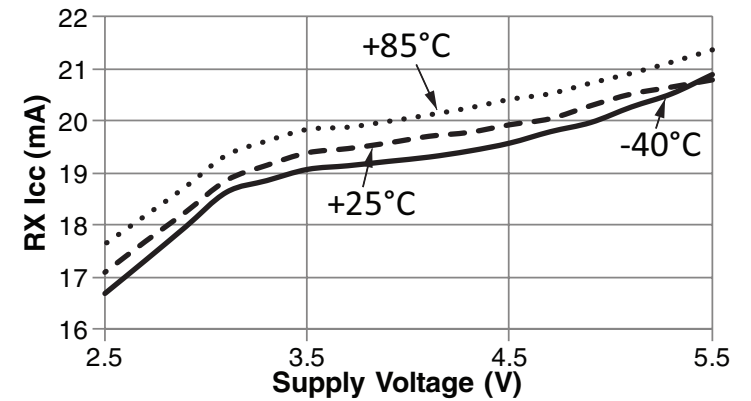
Figure 10: NT Series Transceiver RX Current Consumption vs. Supply Voltage
