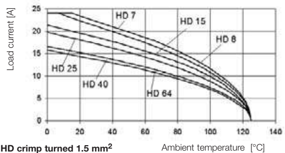
HD crimp turned 1.5 mm 2
