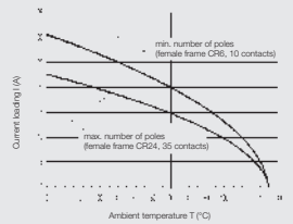
ConCept module CM-5 Conductor H07V-K 4.0 mm²
