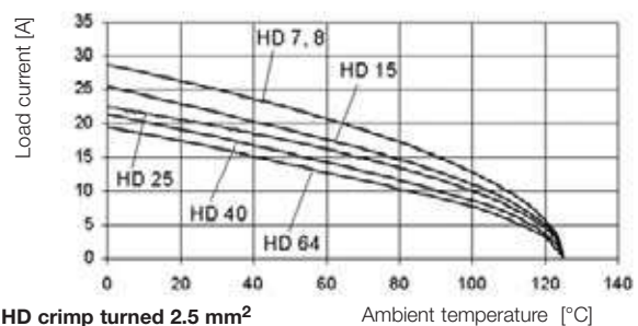
HD crimp turned 2.5 mm 2
