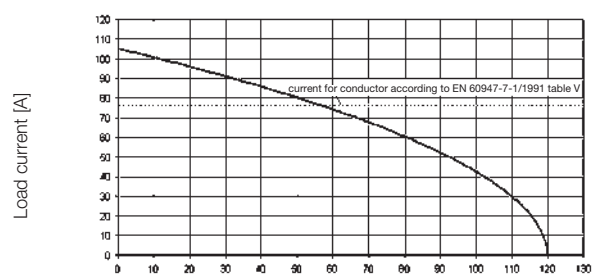
HDC-S4/0-SAS/BAS H07V-K16 Ambient temperature [°C]
