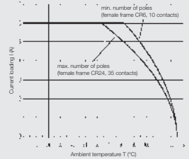
ConCept module CM-5 Conductor H05V-K 0.5 mm²
