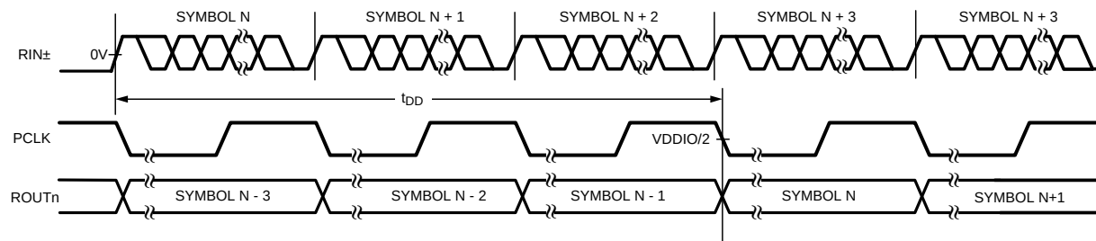
Figure 14. Deserializer Delay
