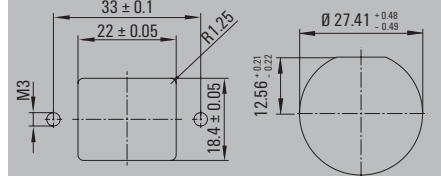
Standardised flange
