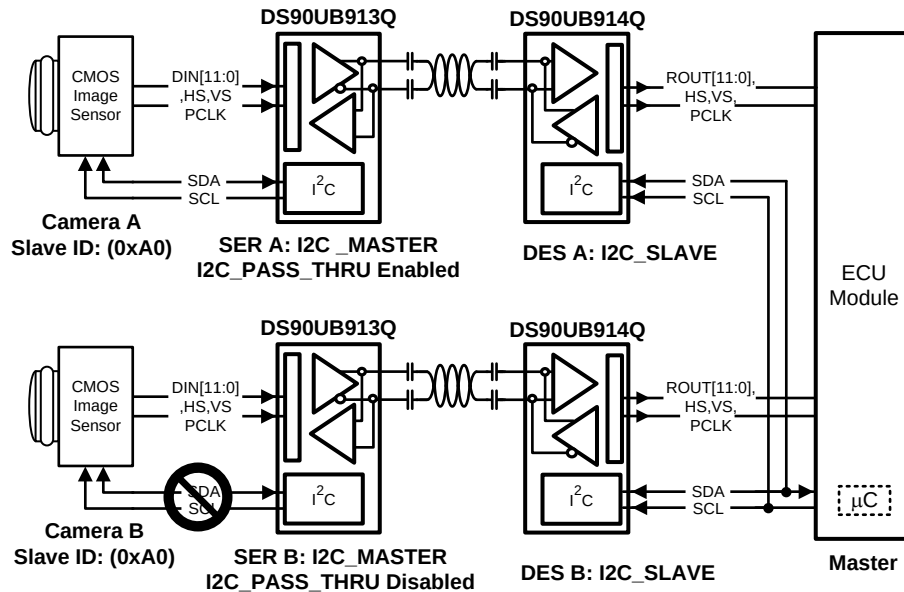
Figure 30. I²C Pass-Through
