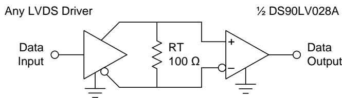
Figure 20. Point-to-Point Application
