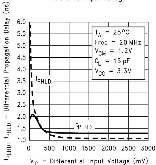
Differential Propagation Delay vs Differential Input Voltage
