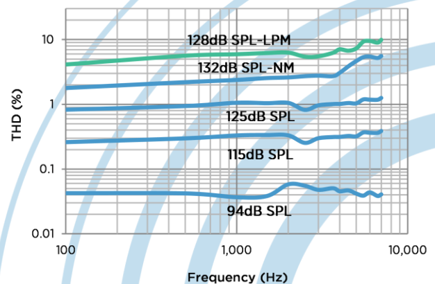
Figure 5: Typical THD vs Input Frequency
