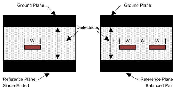
Figure 16. Stripline Topology
