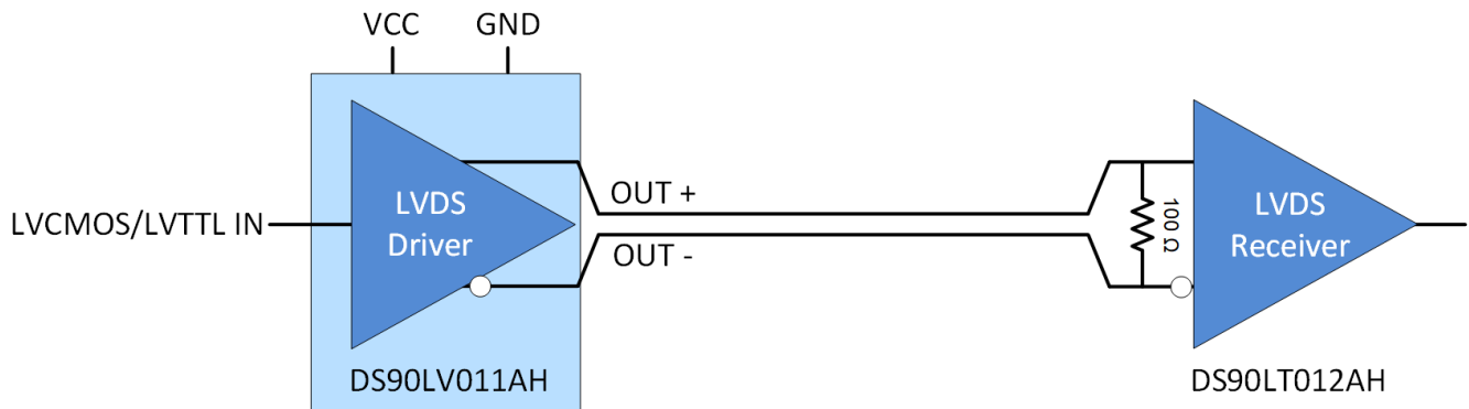
Figure 11. Point-to-Point Application
