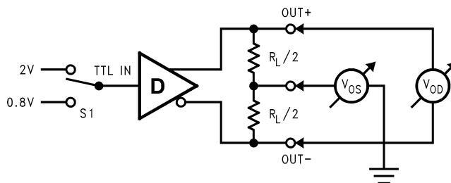
Figure 7. Differential Driver DC Test Circuit
