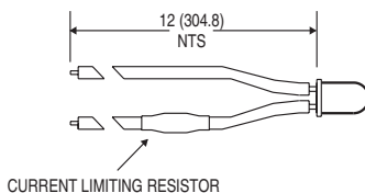
PH25 Outline
