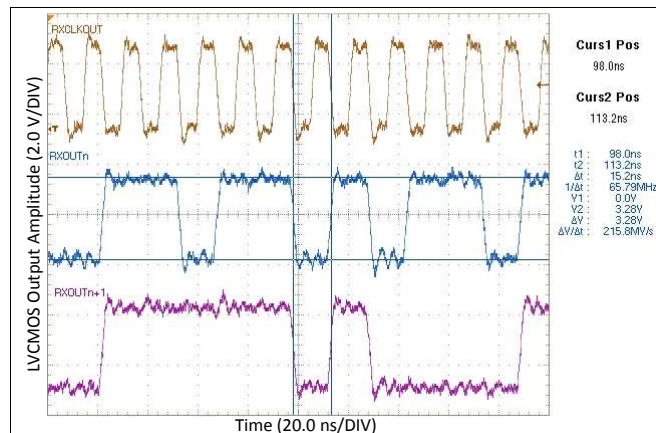
Figure 12. Parallel PRBS-7 on LVCMOS Outputs at 66 MHz
