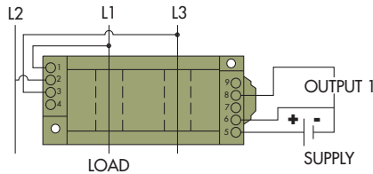
CR6230 CR6231 2 element - 3 Wire, 0 - 5 VDC Output
